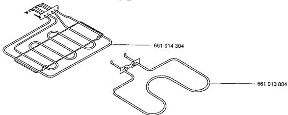
View C
